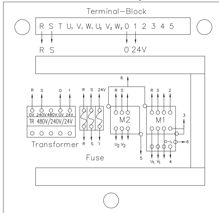
Electrical Schematic for 1 Phase 240V
