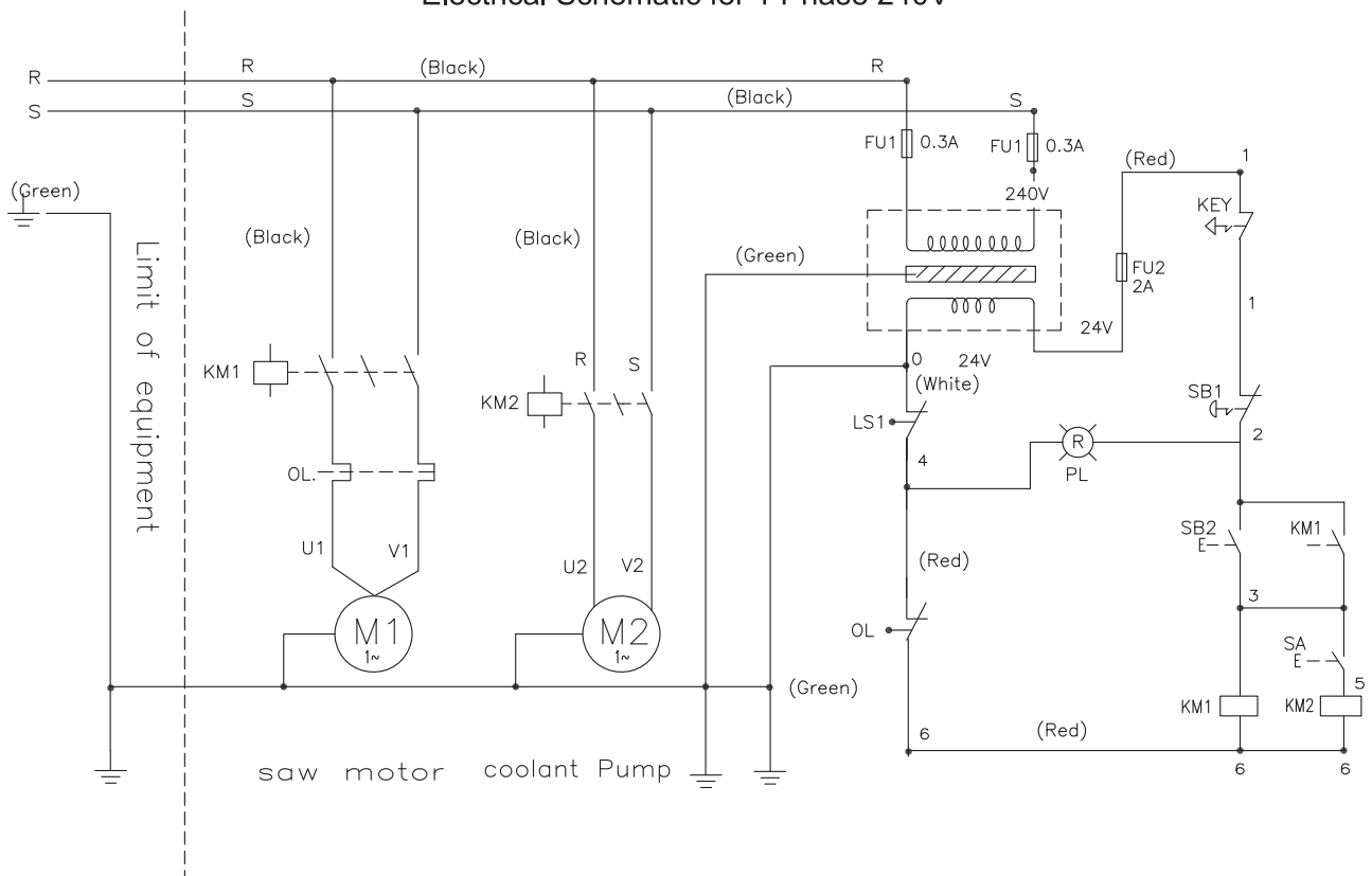
Electrical Schematic for 1 Phase 240V
