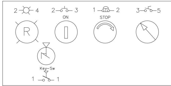
Electrical Panel Layout
