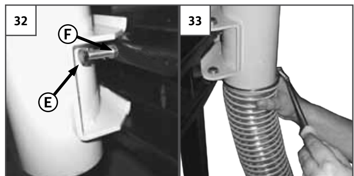
FIGURE 32: ADJUSTING THE BOOM ASSEMBLY
